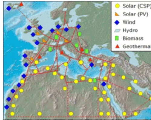
Solar thermal parabolic trough power plant; planned sites for the power plants (concentrated solar power; photovoltaics, water power, biomass and geothermal energy. High-voltage direct-current power lines (red lines); Source: Solar Millennium, TREC.
