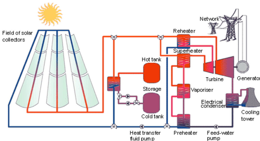
Function scheme of a solar thermal parabolic trough power plant. Source: DLR. [Wording: Field of solar collectors, Hot tank, Storage, Cold tank, Heat transfer fluid pump, Reheater, Superheater,
